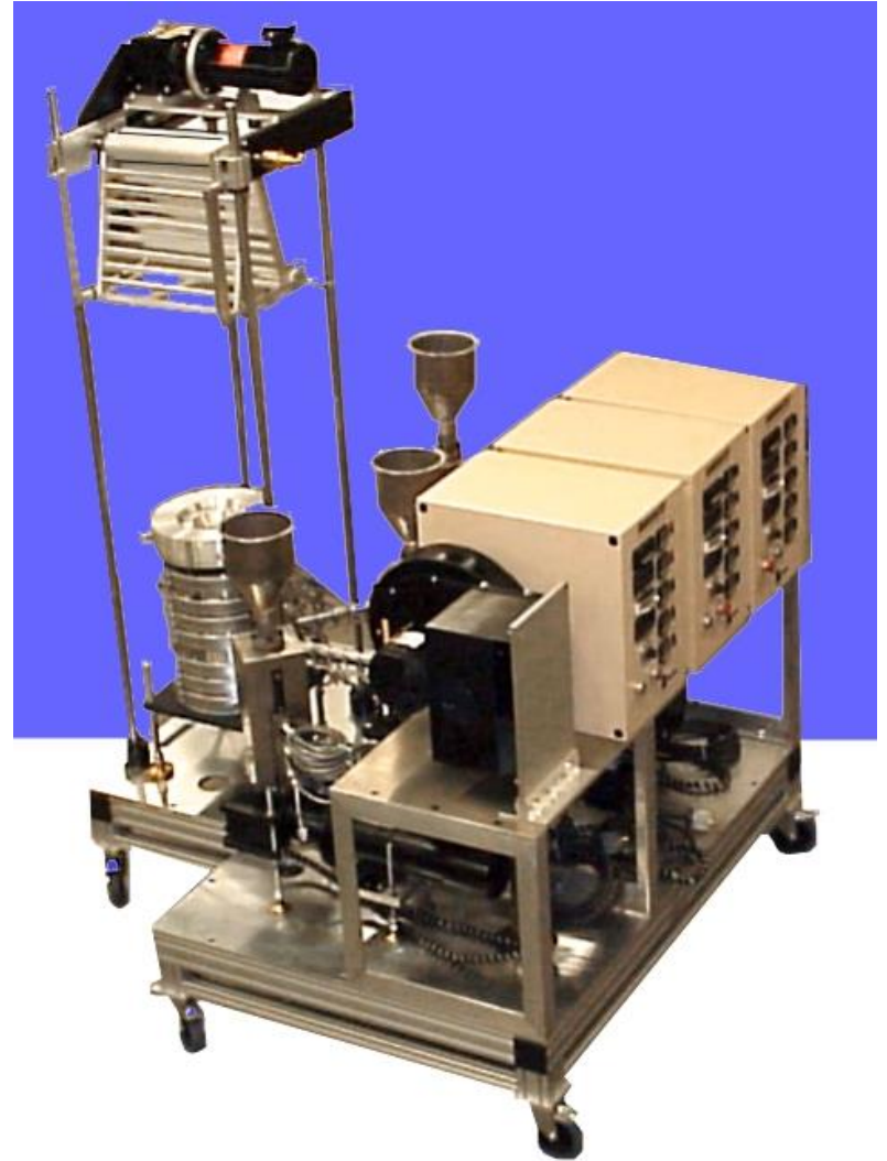
Three RCP-0750 Microtruders for ABCBA structures with adjustable height take up.
