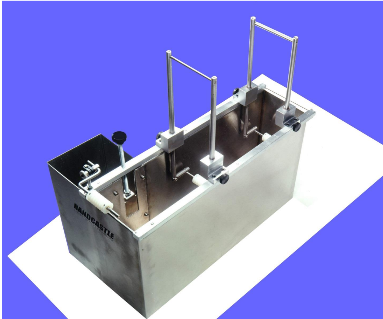
Vertical Water Bath With Guides Adjustable Water Height And Overflow
